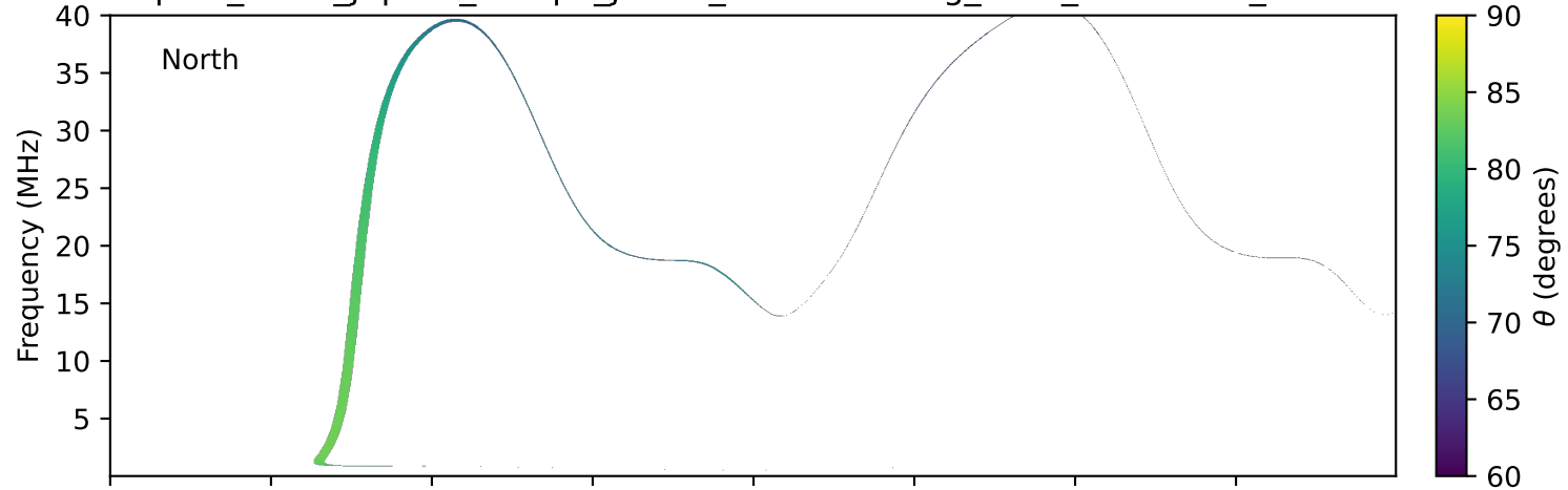
expres_earth_jupiter_europa_jrm33_lossc-wid1deg_3kev_20110825_v11.cdf
