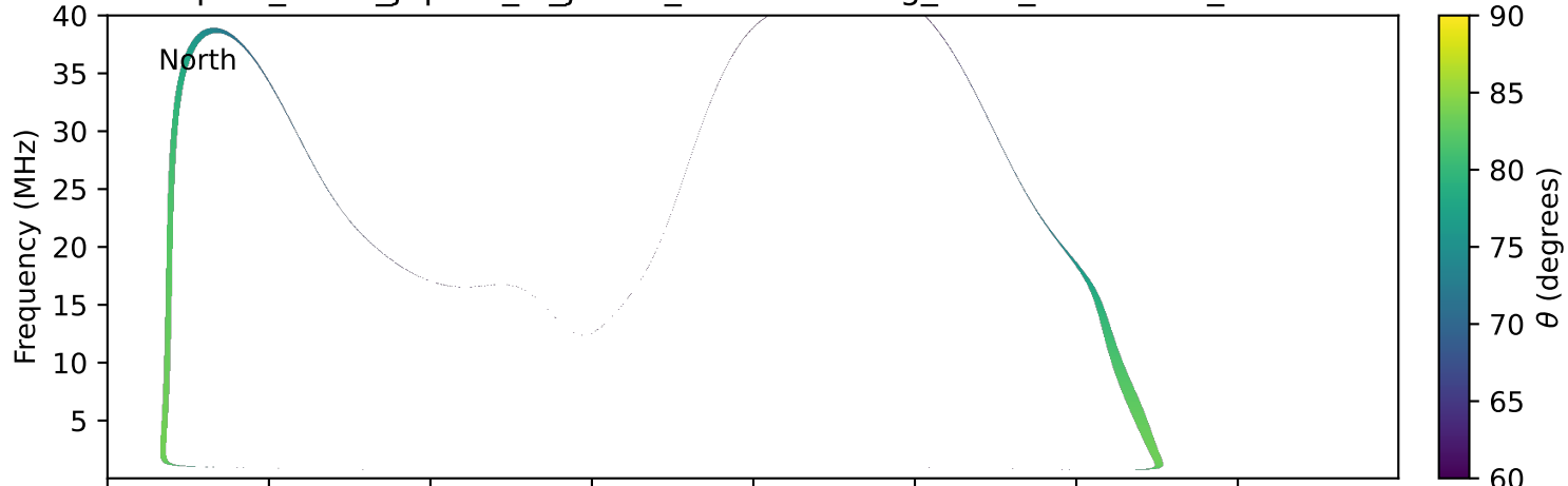
expres_earth_jupiter_io_jrm33_lossc-wid1deg_3kev_20110726_v11.cdf
