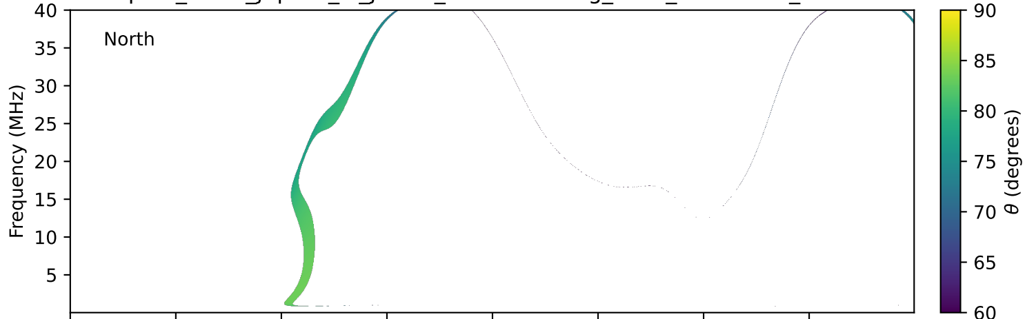
expres_earth_jupiter_io_jrm33_lossc-wid1deg_3kev_20110724_v11.cdf
