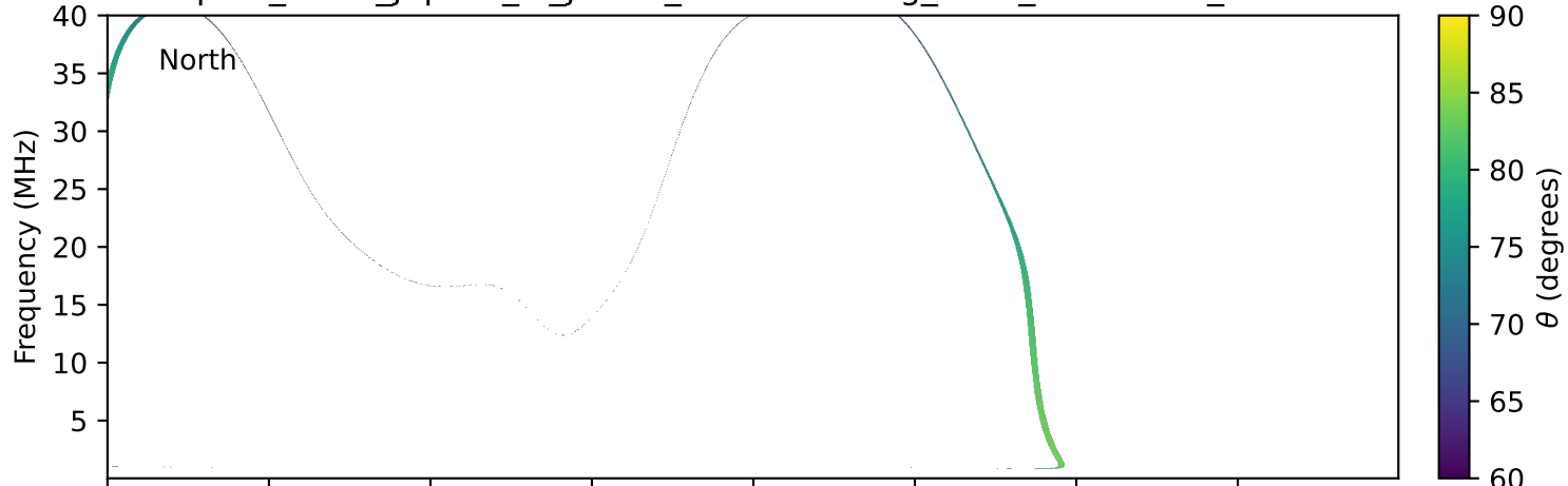
expres_earth_jupiter_io_jrm33_lossc-wid1deg_3kev_20110719_v11.cdf
