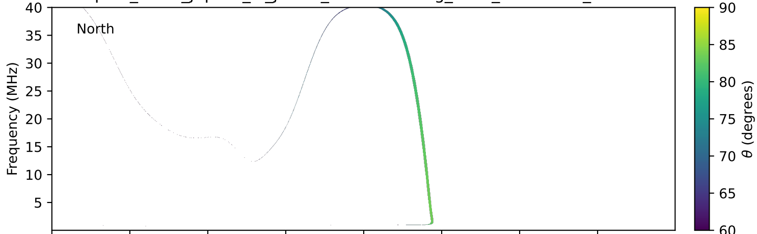
expres_earth_jupiter_io_jrm33_lossc-wid1deg_3kev_20110705_v11.cdf
