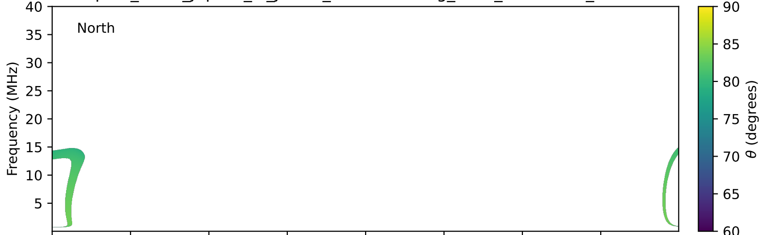
expres_earth_jupiter_io_jrm33_lossc-wid1deg_3kev_20110702_v11.cdf
