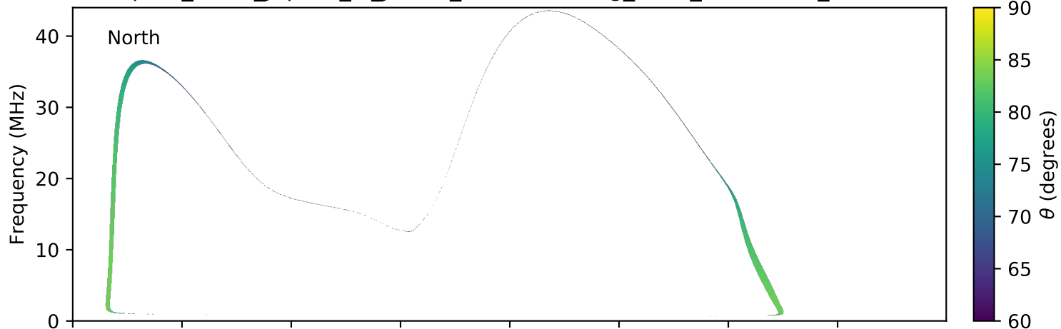
expres_earth_jupiter_io_jrm09_lossc-wid1deg_3kev_20110726_v01.cdf
