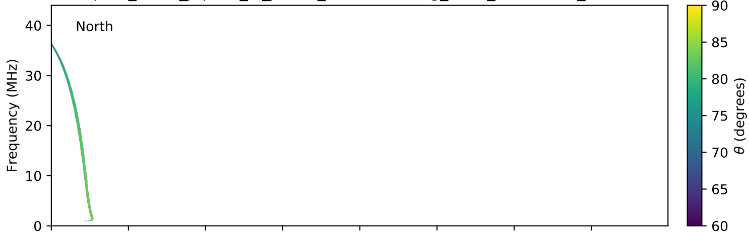
expres_earth_jupiter_io_jrm09_lossc-wid1deg_3kev_20110725_v01.cdf
