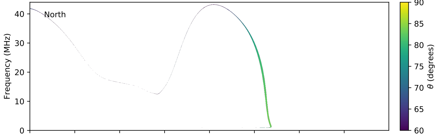
expres_earth_jupiter_io_jrm09_lossc-wid1deg_3kev_20110712_v01.cdf
