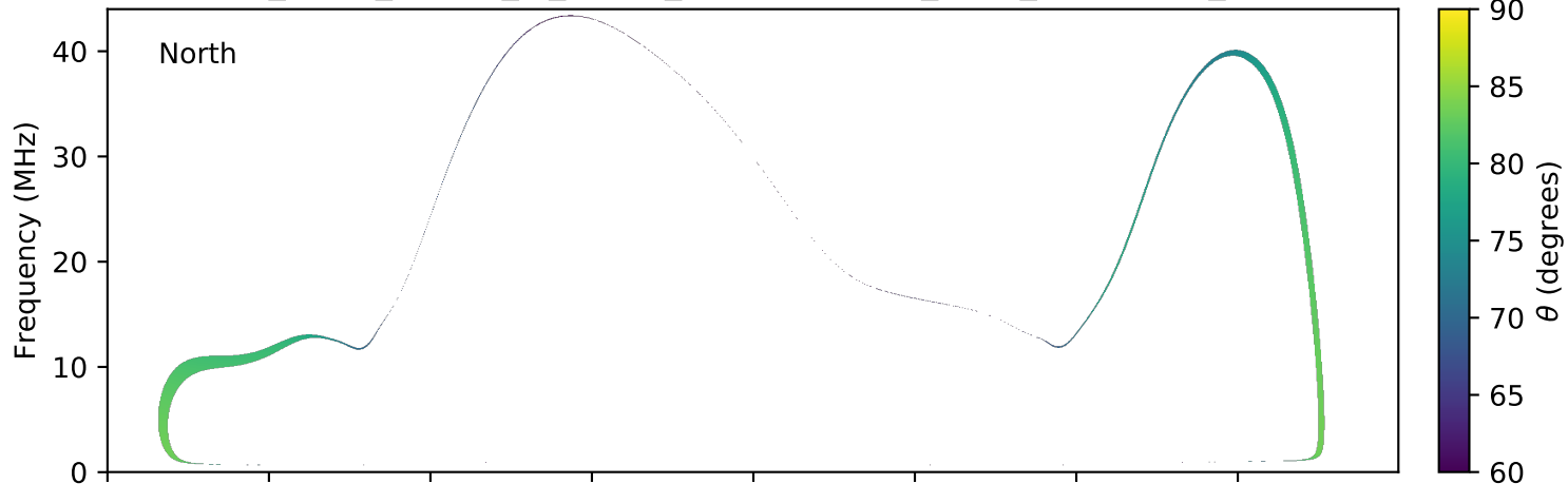
expres_earth_jupiter_io_jrm09_lossc-wid1deg_3kev_20110710_v01.cdf
