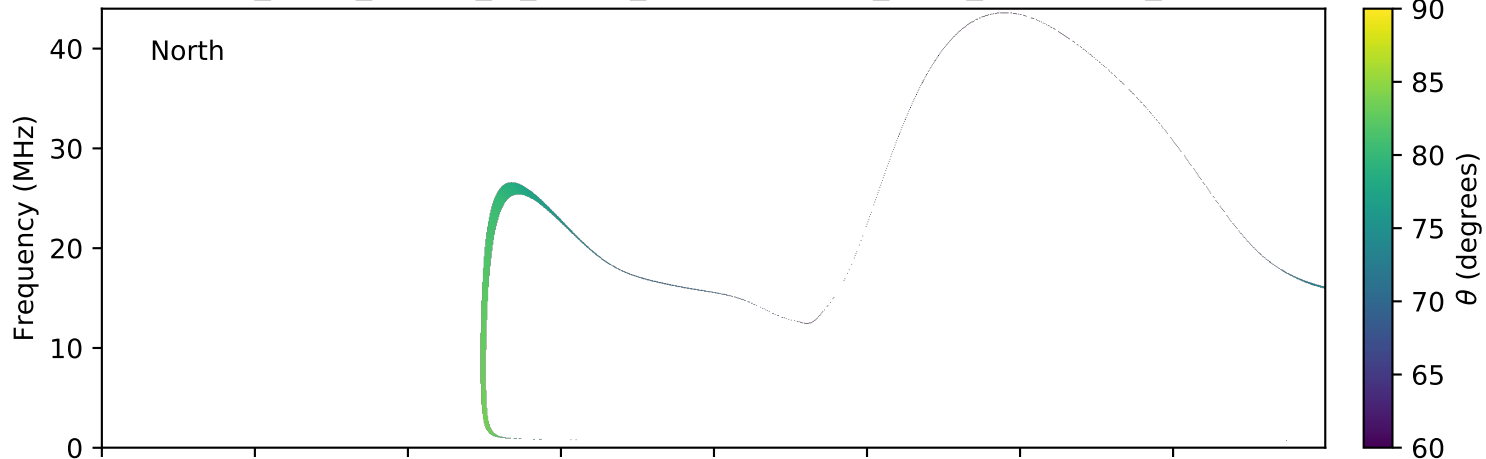
expres_earth_jupiter_io_jrm09_lossc-wid1deg_3kev_20110708_v01.cdf
