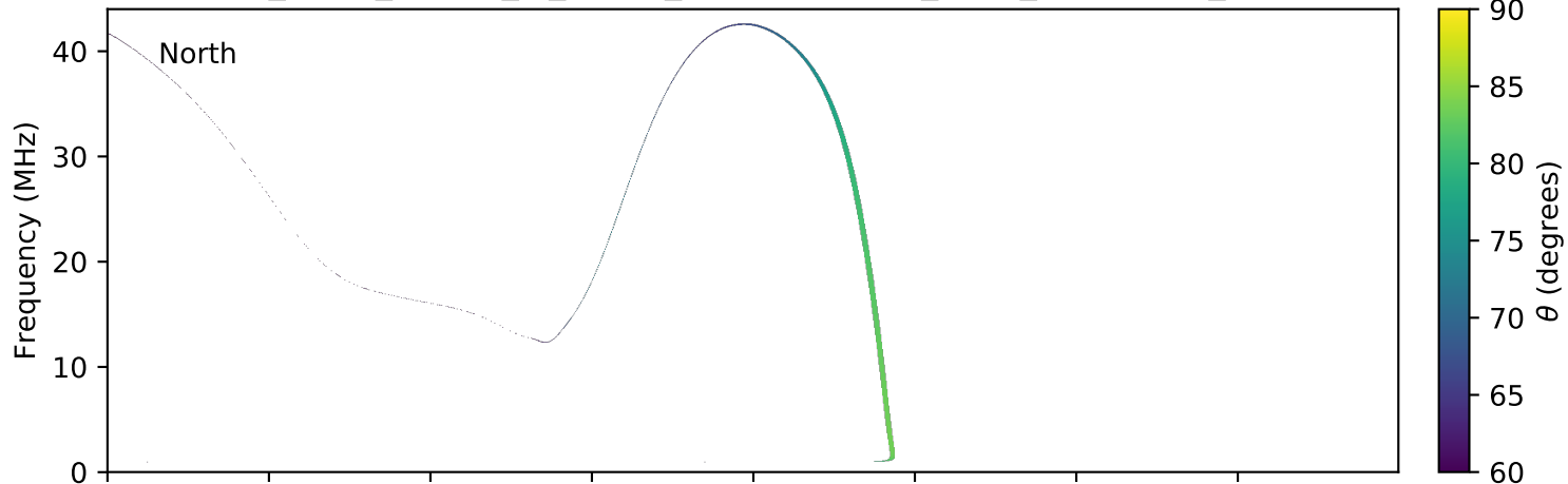
expres_earth_jupiter_io_jrm09_lossc-wid1deg_3kev_20110705_v01.cdf
