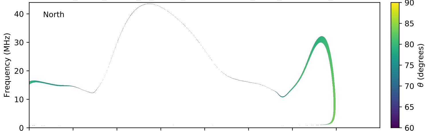
expres_earth_jupiter_io_jrm09_lossc-wid1deg_3kev_20110703_v01.cdf
