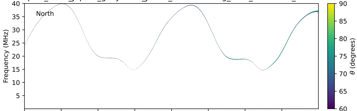
expres_earth_jupiter_ganymede_jrm33_lossc-wid1deg_3kev_20110731_v11.cdf
