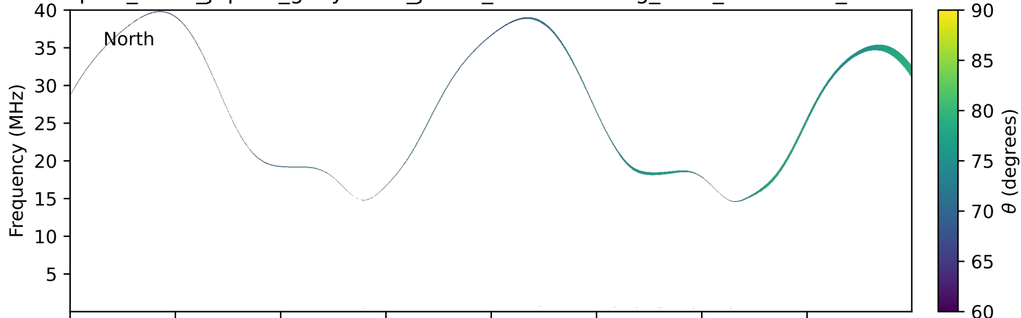
expres_earth_jupiter_ganymede_jrm33_lossc-wid1deg_3kev_20110724_v11.cdf
