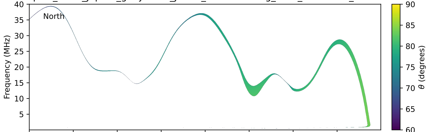
expres_earth_jupiter_ganymede_jrm33_lossc-wid1deg_3kev_20110710_v11.cdf
