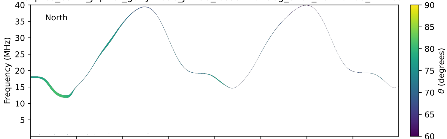
expres_earth_jupiter_ganymede_jrm33_lossc-wid1deg_3kev_20110708_v11.cdf
