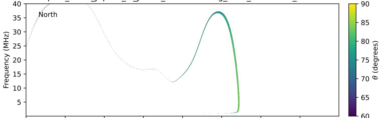
expres_earth_jupiter_io_jrm33_lossc-wid1deg_3kev_20110527_v11.cdf
