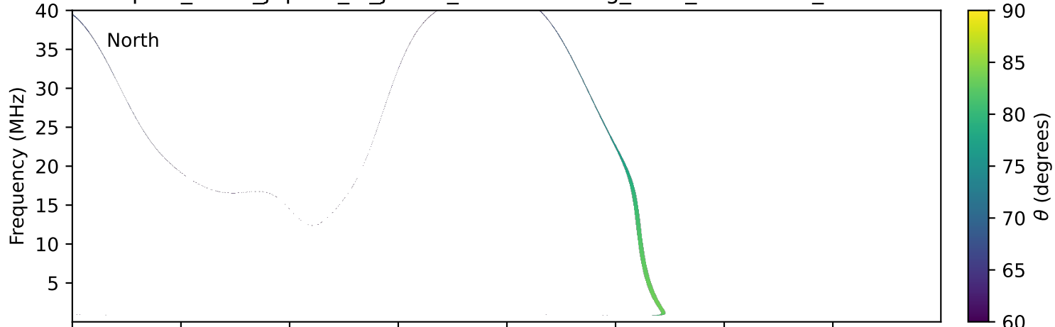
expres_earth_jupiter_io_jrm33_lossc-wid1deg_3kev_20110511_v11.cdf
