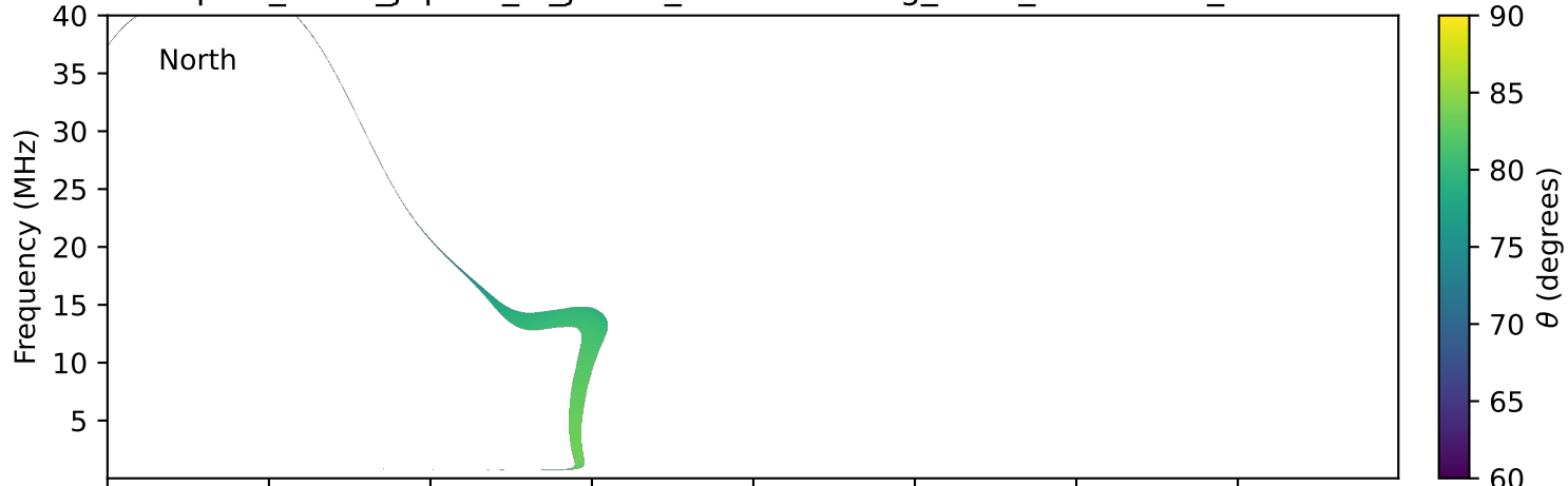
expres_earth_jupiter_io_jrm33_lossc-wid1deg_3kev_20110506_v11.cdf
