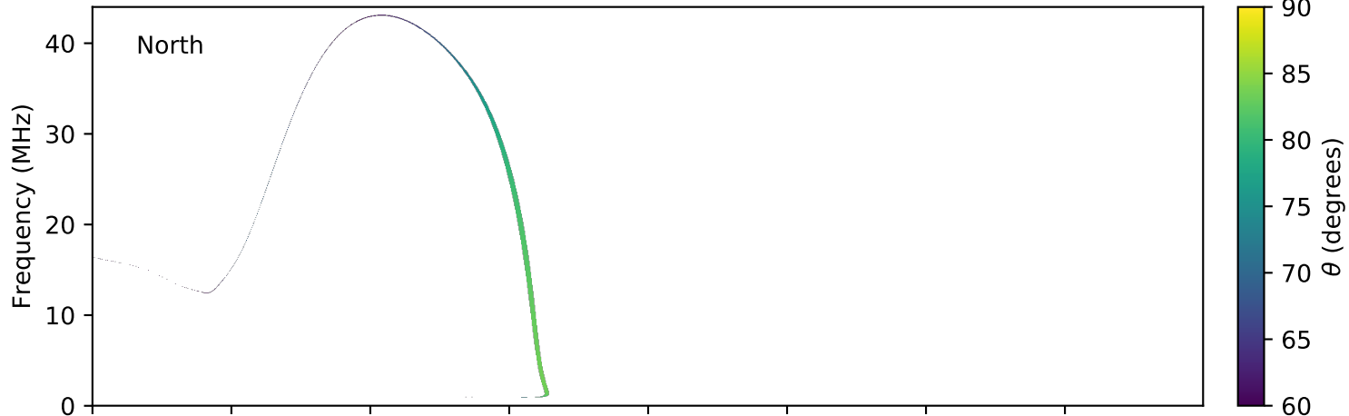
expres_earth_jupiter_io_jrm09_lossc-wid1deg_3kev_20110529_v01.cdf
