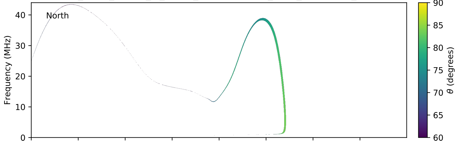
expres_earth_jupiter_io_jrm09_lossc-wid1deg_3kev_20110527_v01.cdf
