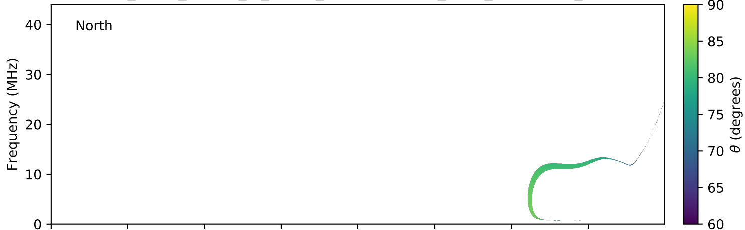
expres_earth_jupiter_io_jrm09_lossc-wid1deg_3kev_20110526_v01.cdf
