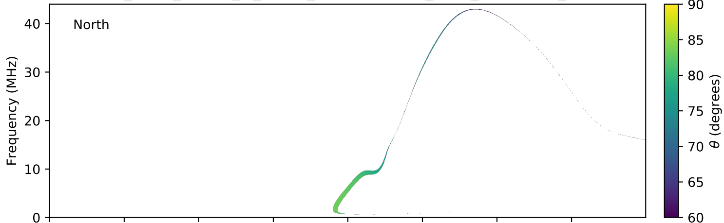
expres_earth_jupiter_io_jrm09_lossc-wid1deg_3kev_20110521_v01.cdf
