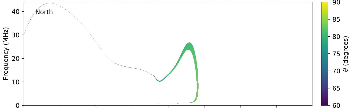
expres_earth_jupiter_io_jrm09_lossc-wid1deg_3kev_20110520_v01.cdf
