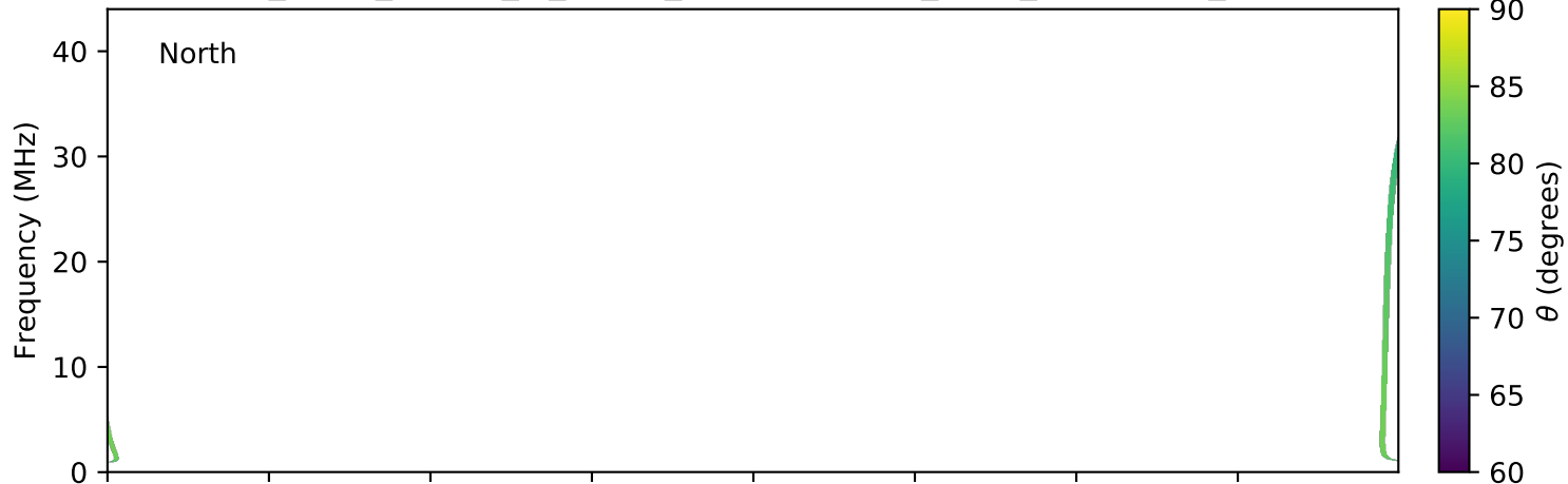
expres_earth_jupiter_io_jrm09_lossc-wid1deg_3kev_20110517_v01.cdf
