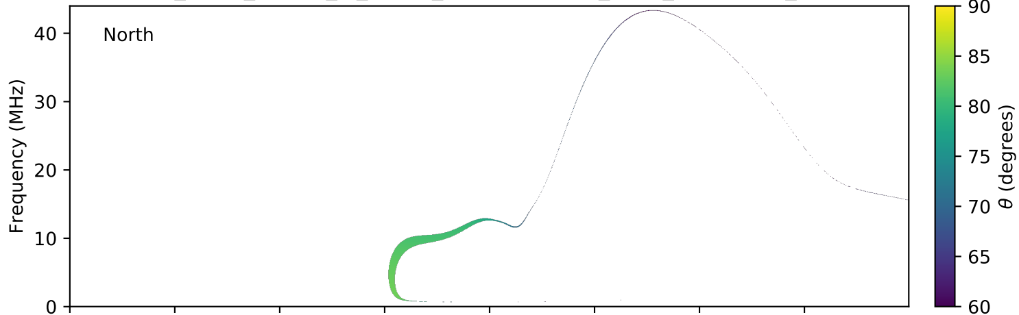
expres_earth_jupiter_io_jrm09_lossc-wid1deg_3kev_20110514_v01.cdf
