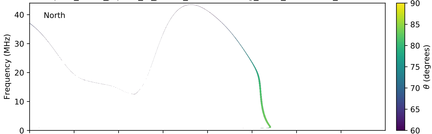
expres_earth_jupiter_io_jrm09_lossc-wid1deg_3kev_20110511_v01.cdf
