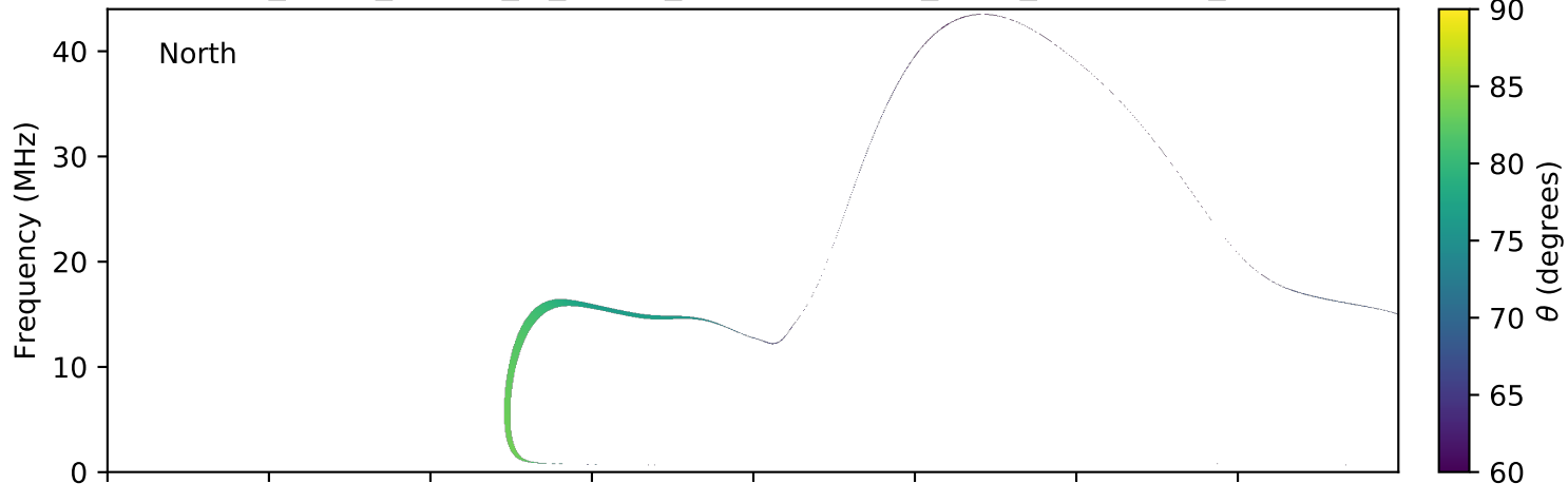
expres_earth_jupiter_io_jrm09_lossc-wid1deg_3kev_20110507_v01.cdf
