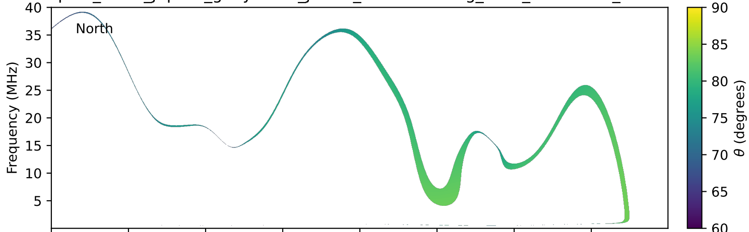
expres_earth_jupiter_ganymede_jrm33_lossc-wid1deg_3kev_20110528_v11.cdf
