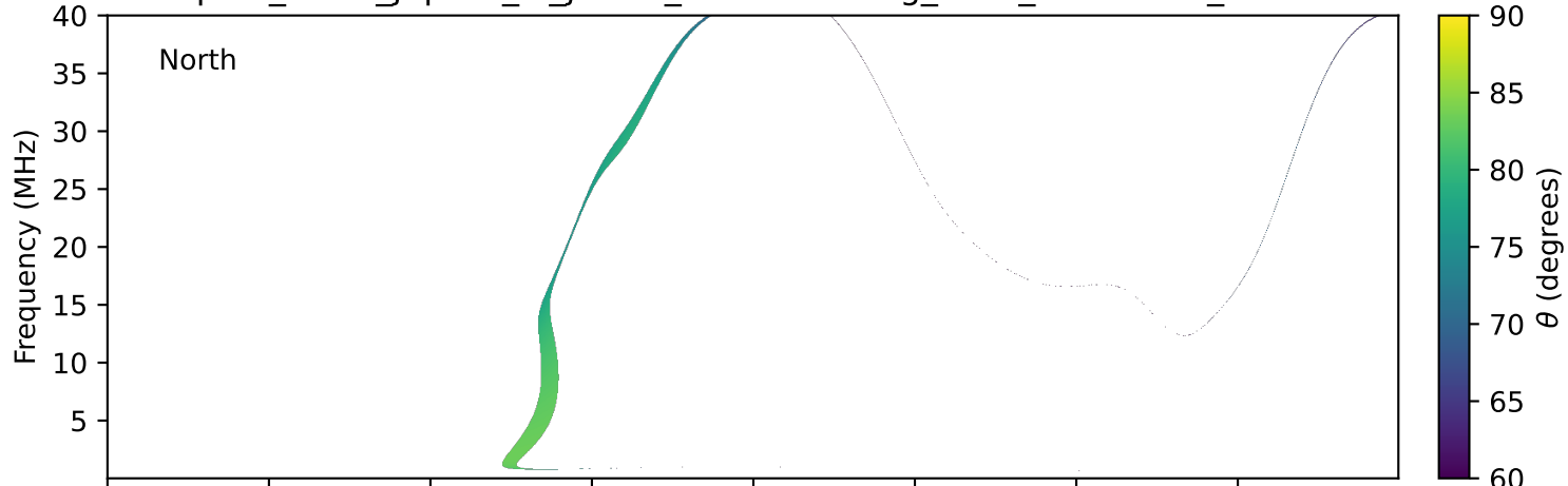
expres_earth_jupiter_io_jrm33_lossc-wid1deg_3kev_20110414_v11.cdf
