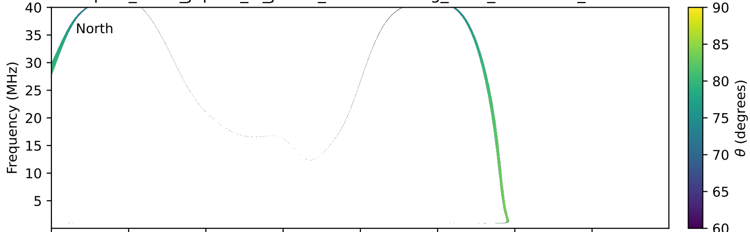
expres_earth_jupiter_io_jrm33_lossc-wid1deg_3kev_20110402_v11.cdf
