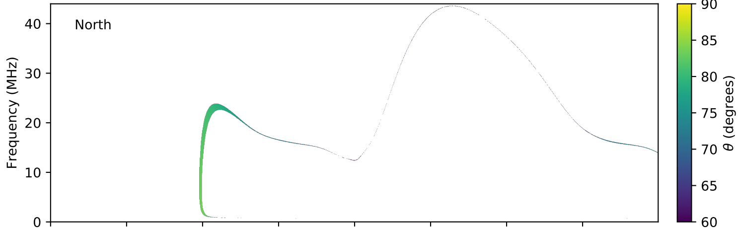
expres_earth_jupiter_io_jrm09_lossc-wid1deg_3kev_20110430_v01.cdf
