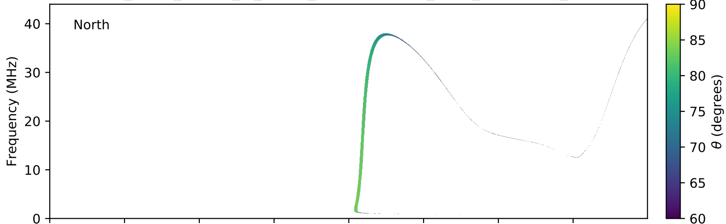
expres_earth_jupiter_io_jrm09_lossc-wid1deg_3kev_20110428_v01.cdf
