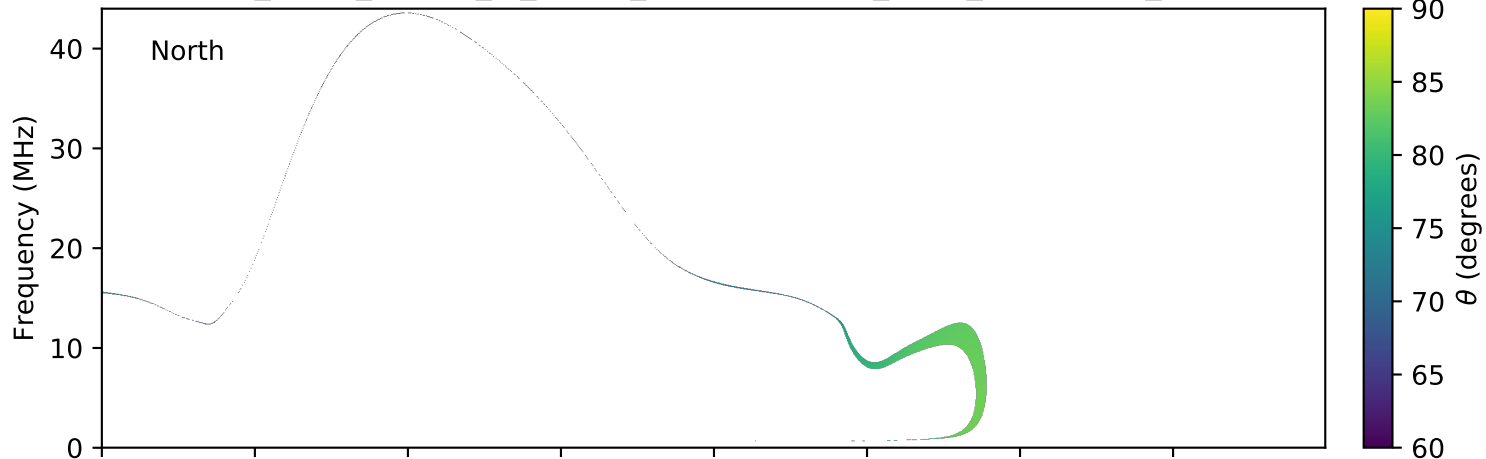
expres_earth_jupiter_io_jrm09_lossc-wid1deg_3kev_20110418_v01.cdf
