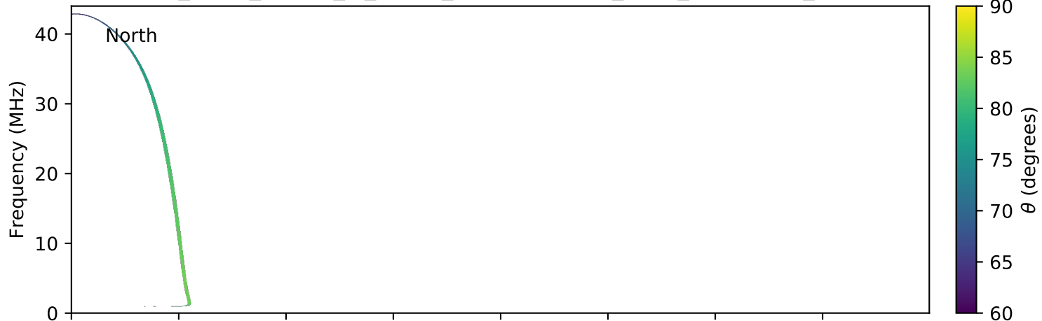
expres_earth_jupiter_io_jrm09_lossc-wid1deg_3kev_20110415_v01.cdf
