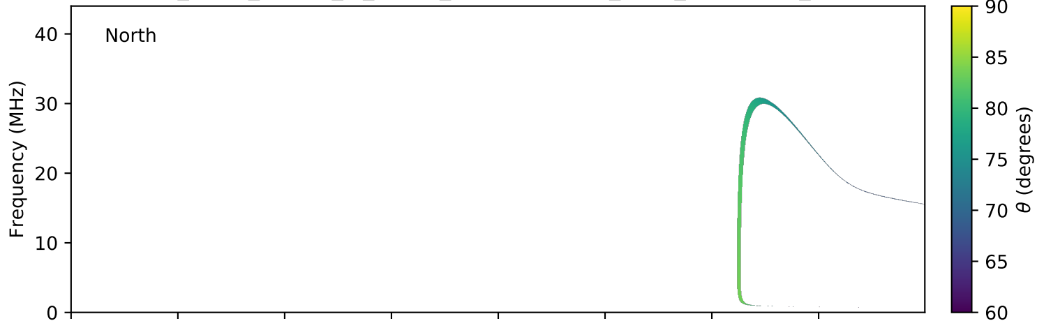
expres_earth_jupiter_io_jrm09_lossc-wid1deg_3kev_20110410_v01.cdf
