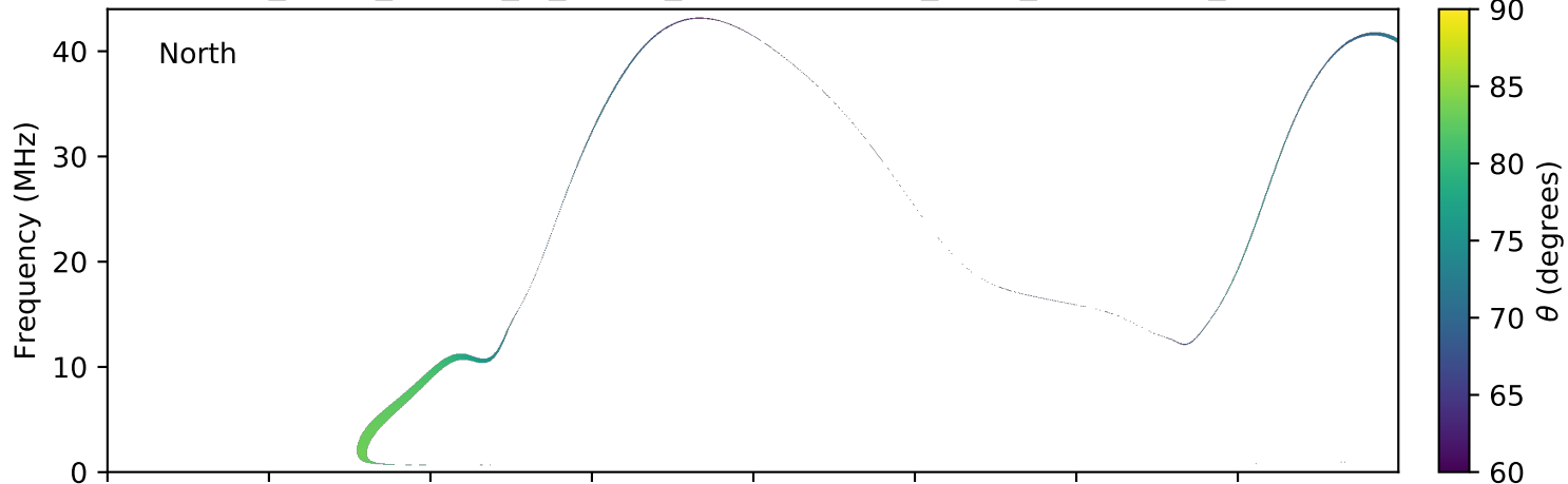
expres_earth_jupiter_io_jrm09_lossc-wid1deg_3kev_20110407_v01.cdf
