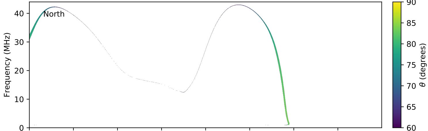
expres_earth_jupiter_io_jrm09_lossc-wid1deg_3kev_20110402_v01.cdf
