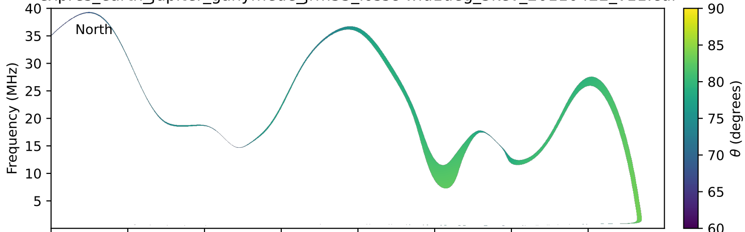
expres_earth_jupiter_ganymede_jrm33_lossc-wid1deg_3kev_20110422_v11.cdf
