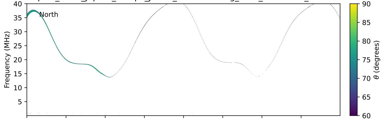
expres_earth_jupiter_europa_jrm33_lossc-wid1deg_3kev_20110412_v11.cdf
