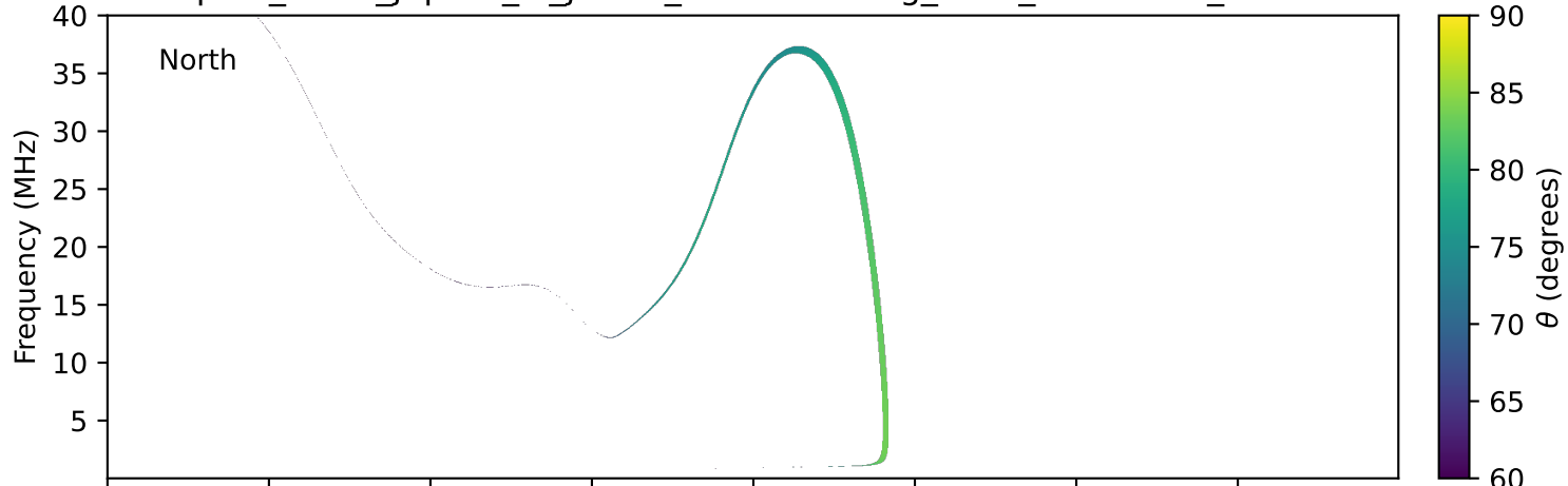
expres_earth_jupiter_io_jrm33_lossc-wid1deg_3kev_20110319_v11.cdf
