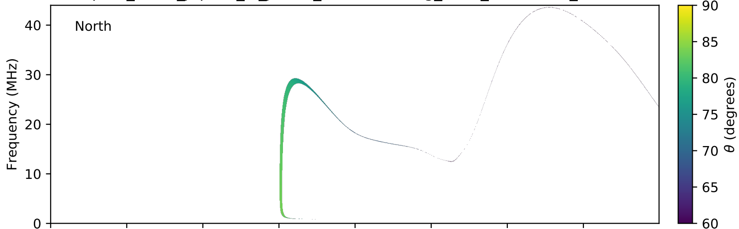
expres_earth_jupiter_io_jrm09_lossc-wid1deg_3kev_20110329_v01.cdf
