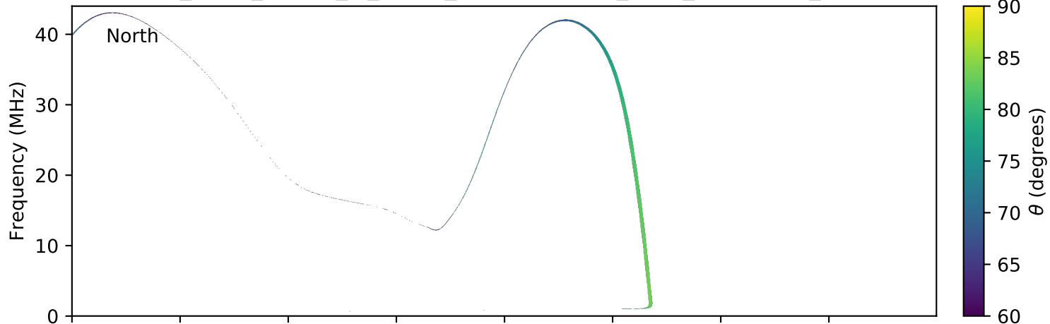
expres_earth_jupiter_io_jrm09_lossc-wid1deg_3kev_20110326_v01.cdf
