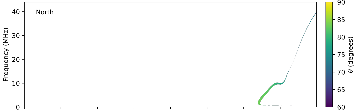
expres_earth_jupiter_io_jrm09_lossc-wid1deg_3kev_20110325_v01.cdf
