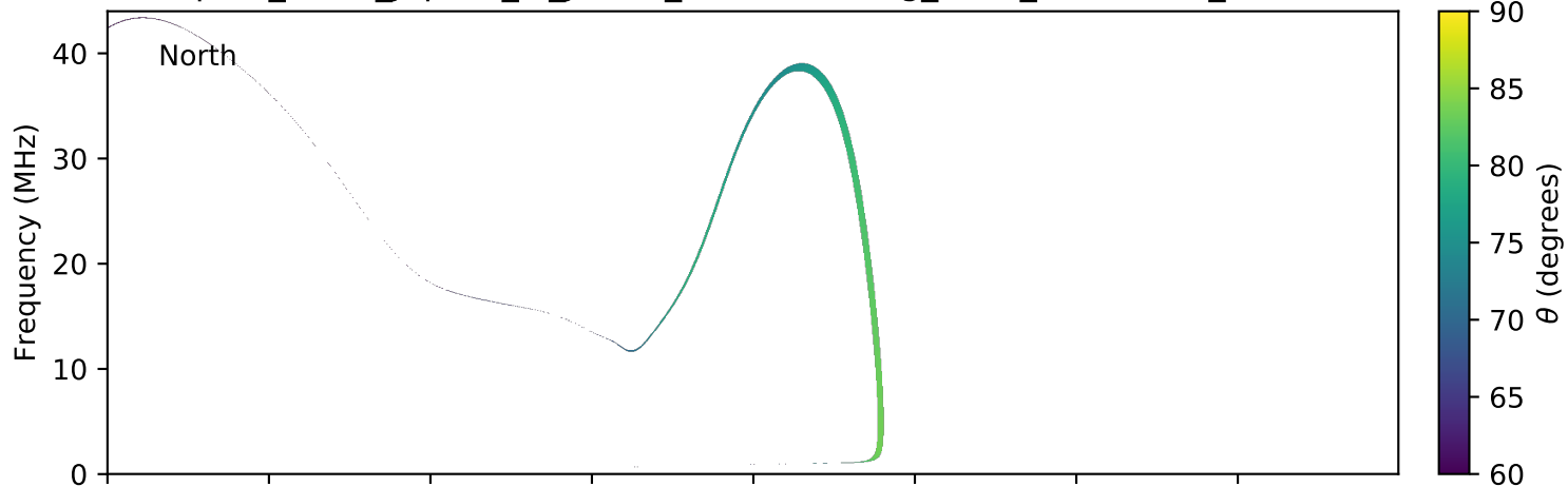
expres_earth_jupiter_io_jrm09_lossc-wid1deg_3kev_20110319_v01.cdf
