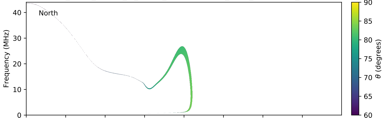
expres_earth_jupiter_io_jrm09_lossc-wid1deg_3kev_20110312_v01.cdf
