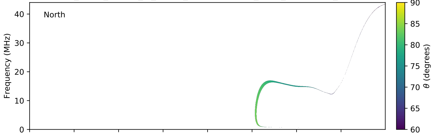
expres_earth_jupiter_io_jrm09_lossc-wid1deg_3kev_20110311_v01.cdf
