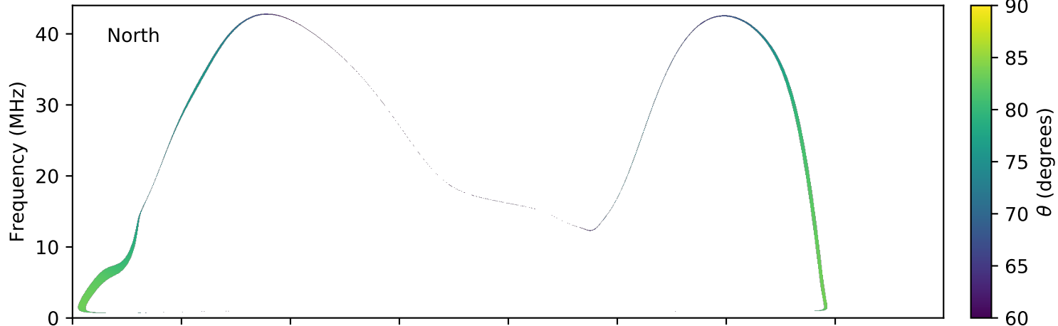
expres_earth_jupiter_io_jrm09_lossc-wid1deg_3kev_20110301_v01.cdf
