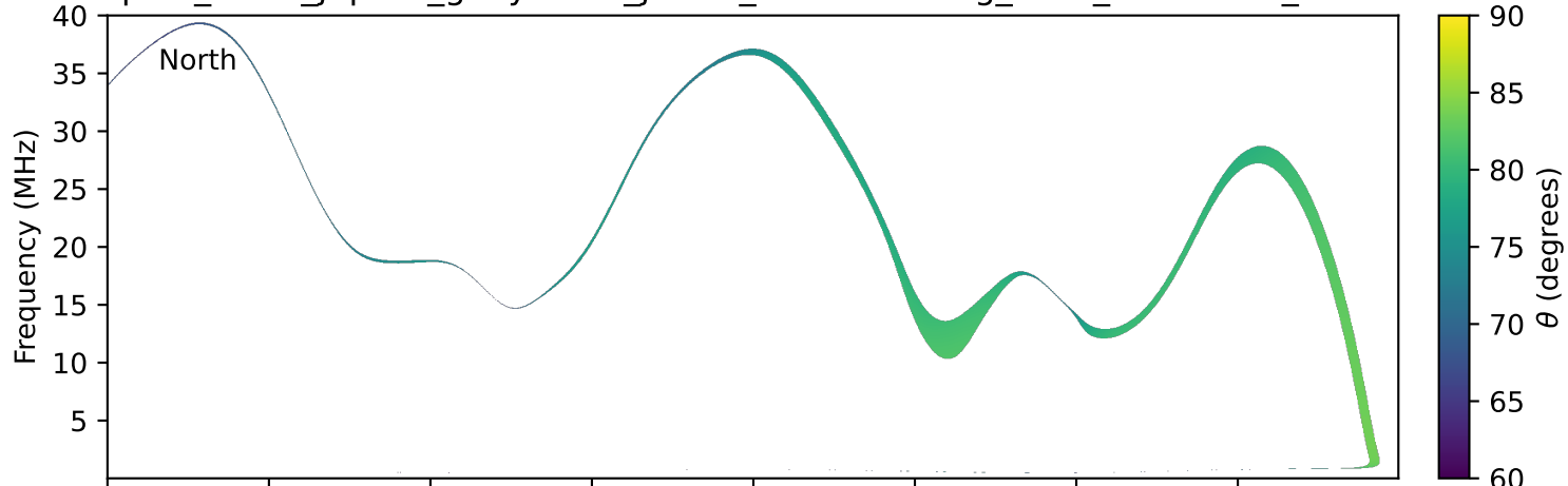
expres_earth_jupiter_ganymede_jrm33_lossc-wid1deg_3kev_20110317_v11.cdf
